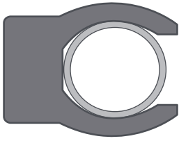
H-Helicoil spring type radial and face type seal from 1/16 up to 1/2 inch
