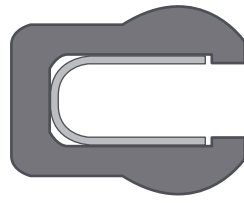
U-Spring type radial and face type seal from 1/16 up to 1/2 inch
