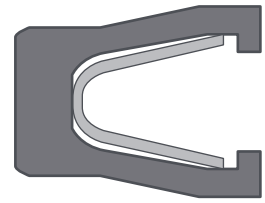
V-Spring type radial and face type seal from 1/16 up to 1/2 inch
